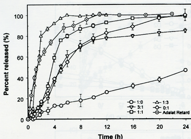
Fig. 5. Dissolution profiles of nifedipine solid dispersions (nifedipine: HPMC = 1:1) from matrix tablets with various ratios of lactose and dicalcium phosphate matrix granules (○: 1:0; ▽: 3:1; □: 1:1; △: 1:3; ◇: 0:1; ⊙: Adalat Retard®).
