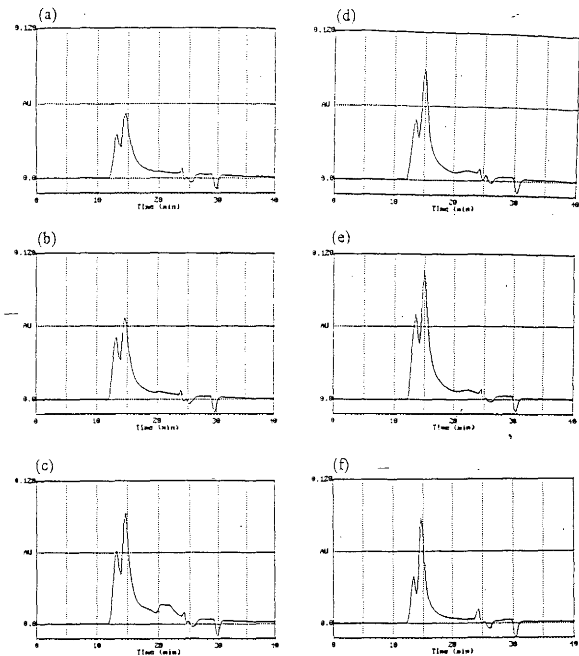
Fig. 6. Size-exclusion chromatography of various preparations of collagen.-Peak maximum ratio = (oligomer/monomer). (a) A/A, 0.68; (b) A/N, 0.77; (c) H/H, 0.65; (d) H/A, 0.35; (e) H/N, 0.62; (f) standard, 0.34.
