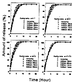
Figure 3. The release profiles of etofibrate from pellets coated with 5.0%
