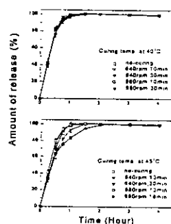
Figure 1. The release profiles of etofibrate from pellets with no coating.
